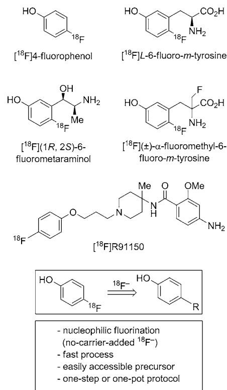
Scheme 1. Importance of the [ 18 F]4-fluorophenol motif for positron emission tomography.
