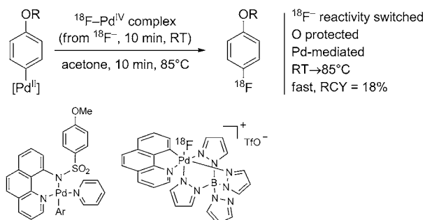
Strategy 2: phenol umpolung (this work)
